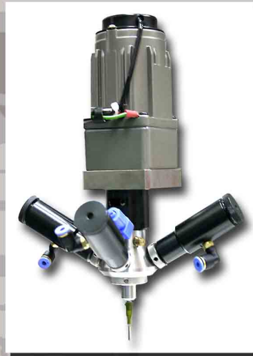
Motor drive dynamic mixer.
